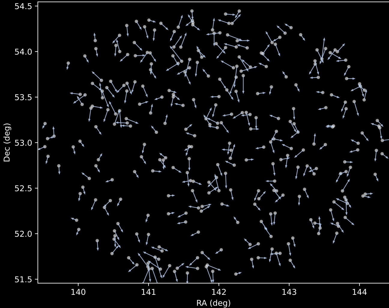
APOGEE DR17 Cluster 1 Proper Motion Vectors (n=309)
