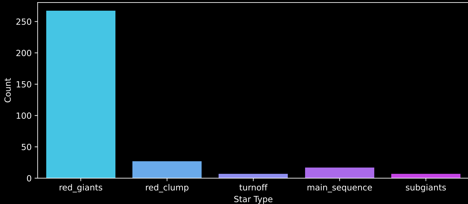
APOGEE DR17 Field: [140-06] Count plot of Star Type
