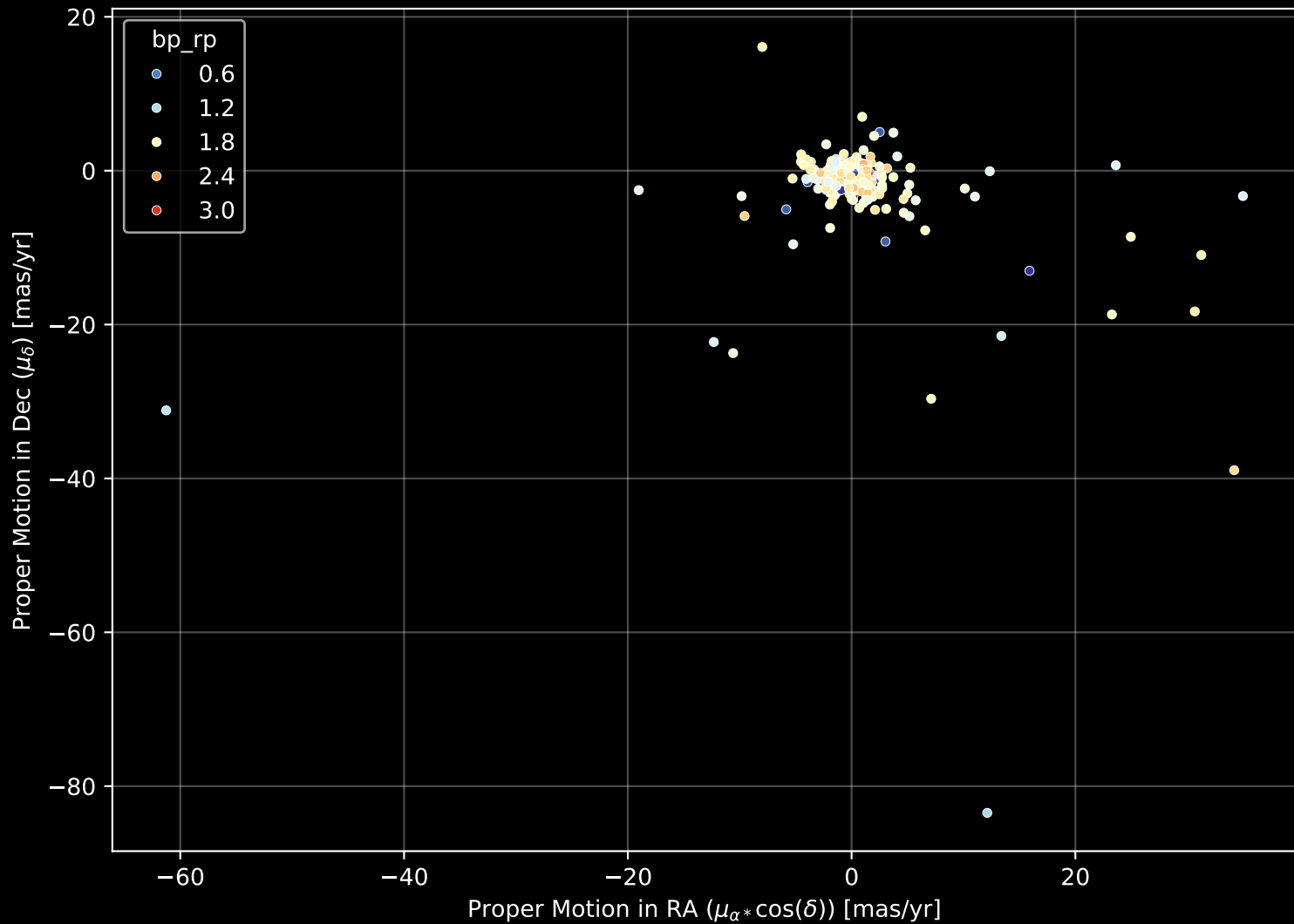
APOGEE DR17 Field: [140-06] Proper Motion Diagram (n= 325)
