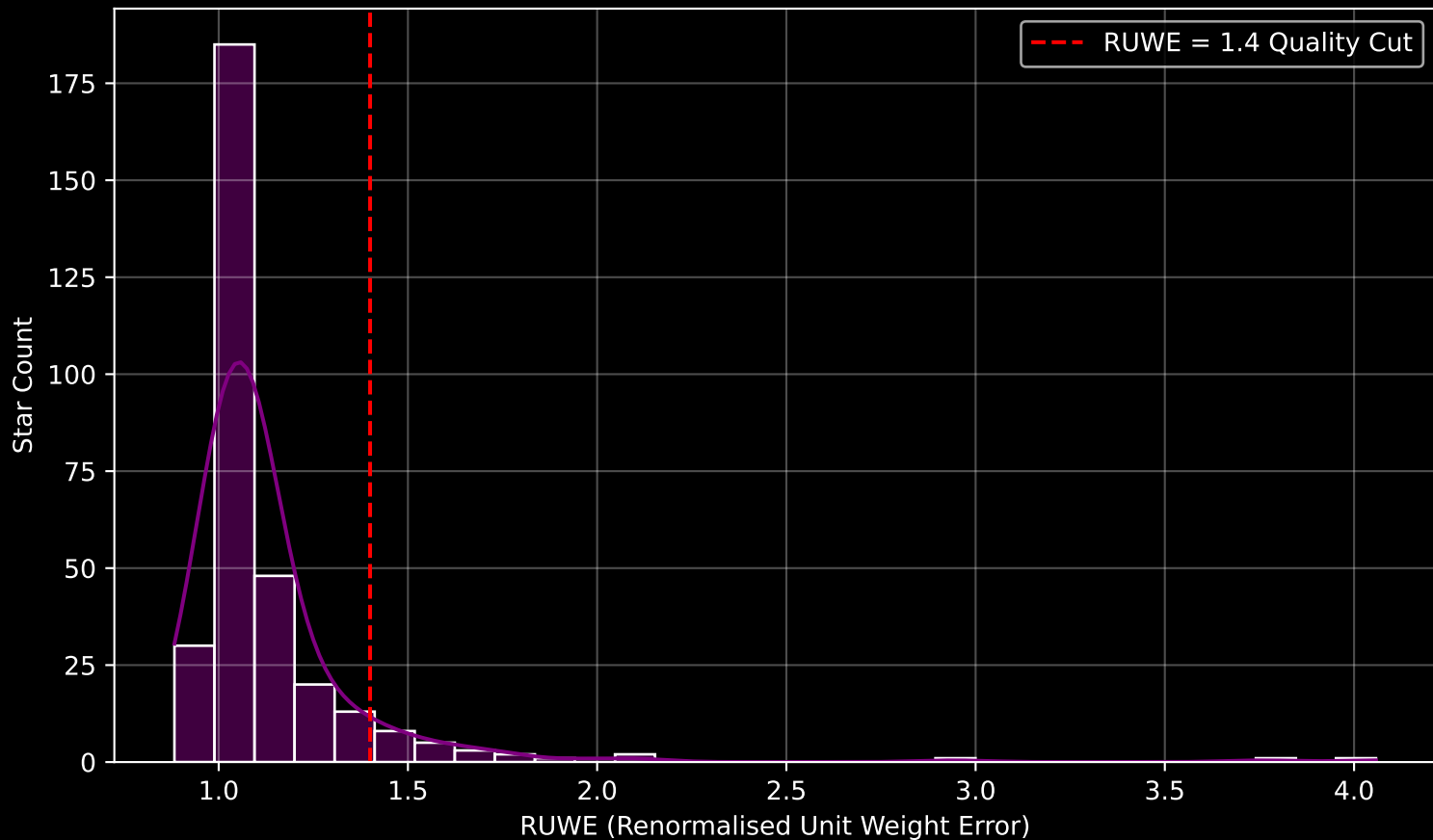
GAPOGEE DR17 Field [140-06] RUWE Distribution (n= 320)
