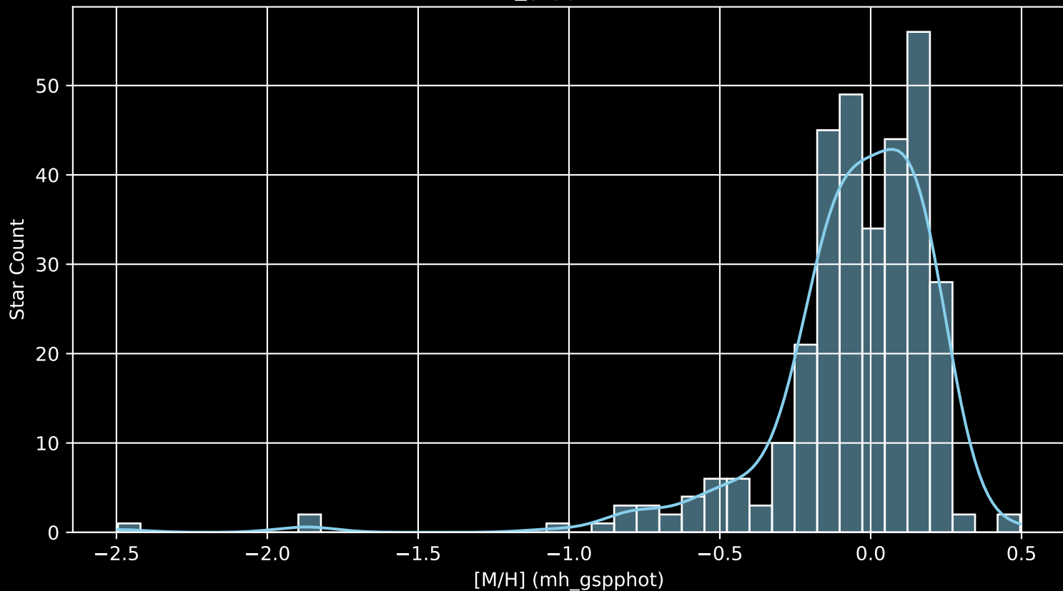
APOGEE DR17 Field: [140-06 [M/H] (mh_gspphot) (n= 323)
