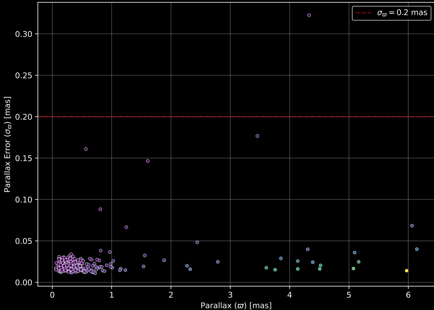
APOGEE DR17 Field: [140-06] Parallax Quality (n= 325)
