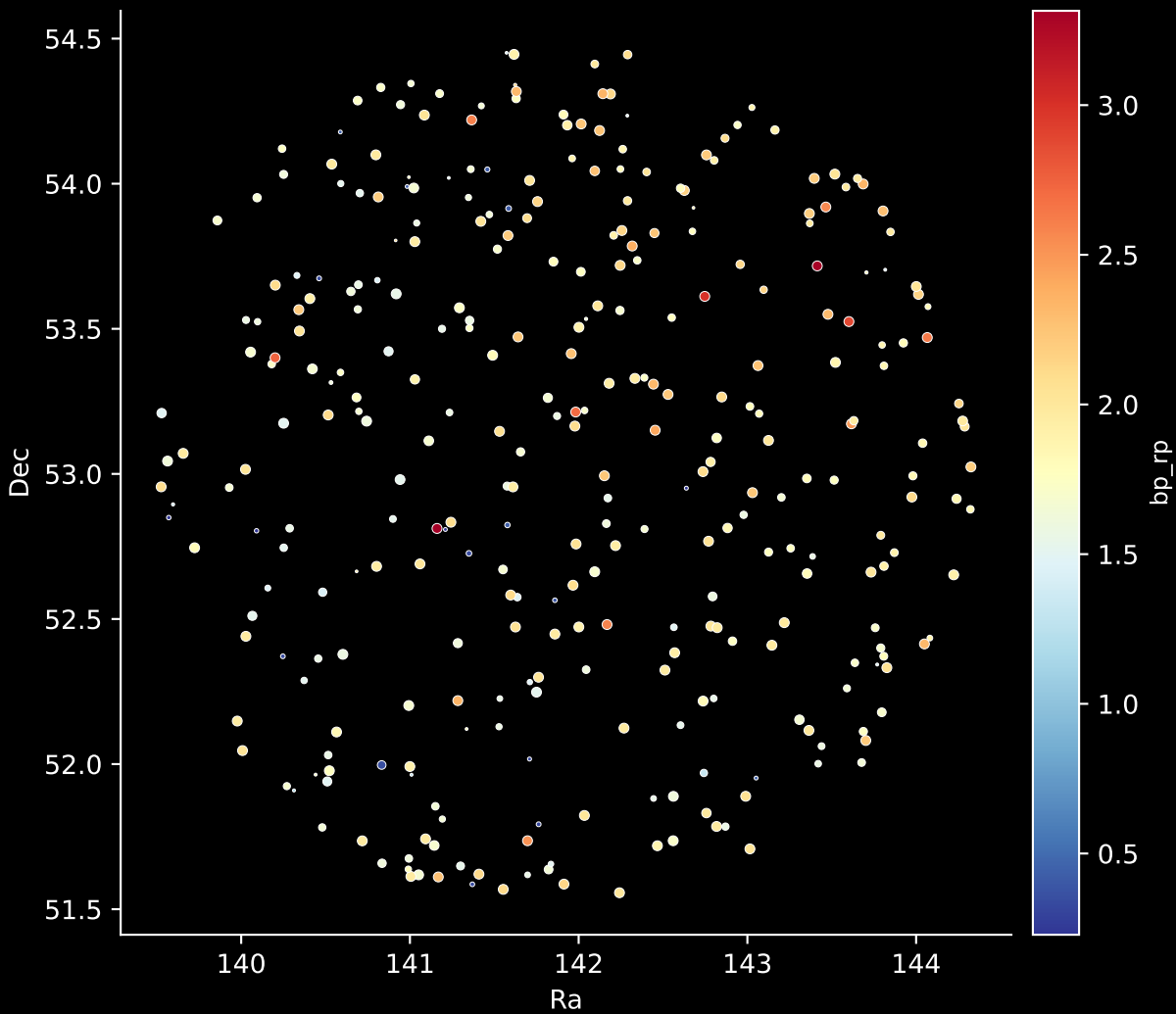
APOGEE DR17 Field: [140-06] Stars: 325
